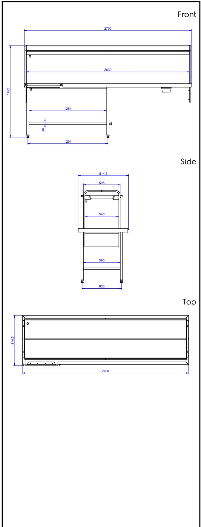
Handling System Sorting Table Right to Left, 2700x800mm
